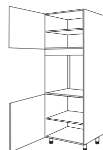
Armoire four 2 portes, 1 tablette amovible Code 005779
